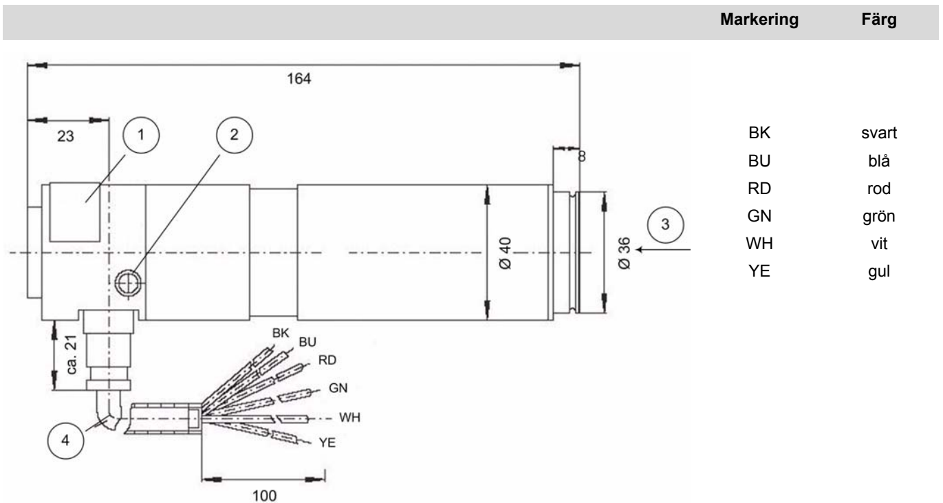
Fig. 8-13 Flamsensor FFS 05
