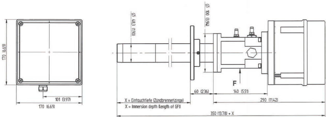
Fig. 4 Dimensions of GFI48 pilot burner Ex-Zone 2
