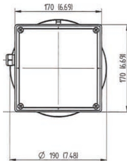
Fig. 10 Dimensions integrated power unit Ex-Zone 2
